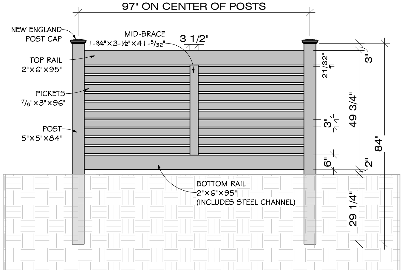
Fence Elevation
