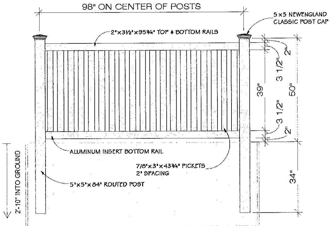
Fence Elevation:
